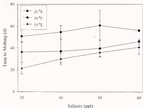
Figure 2. Mean ( \pm SE) time to molting to the first juvenile stage (in days) of Limulus polyphemus at 25 °C, 30 °C, and 33 °C and 30, 40, 50, and 60 ppt. Sample sizes are provided in Table 2.
